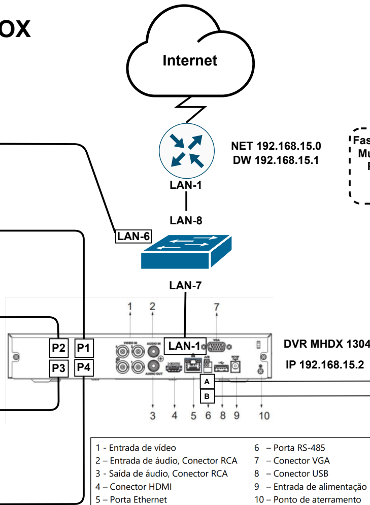
Figura 1 - Painel MHDX 1304
